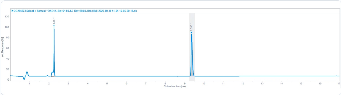
HPLC Chromatogram · Retention Time 2.257, 9.355 min
