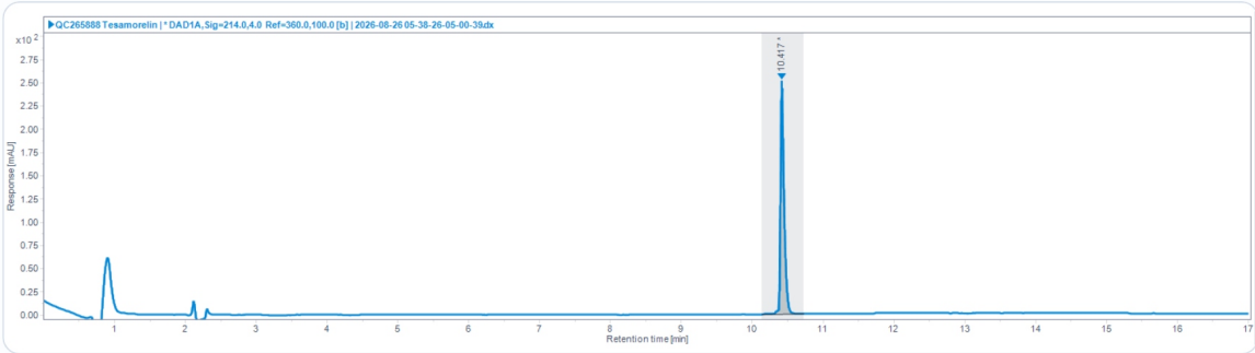
HPLC Chromatogram · Retention Time 10.417 min
