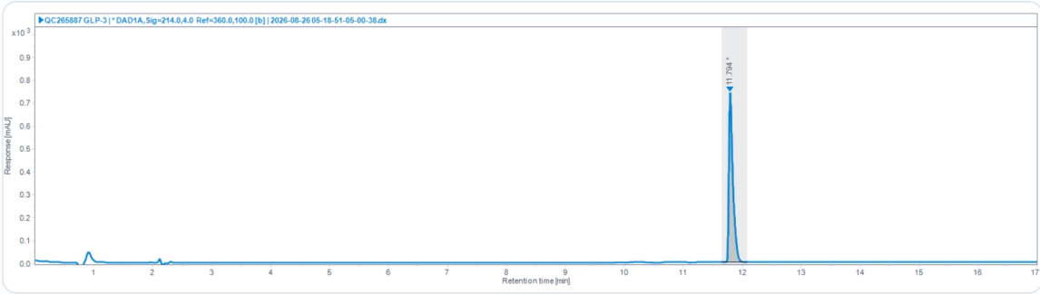
HPLC Chromatogram · Retention Time 11.794 min
