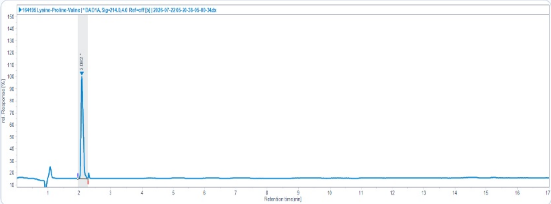
HPLC Chromatogram (Retention Time: 2.082 min)
