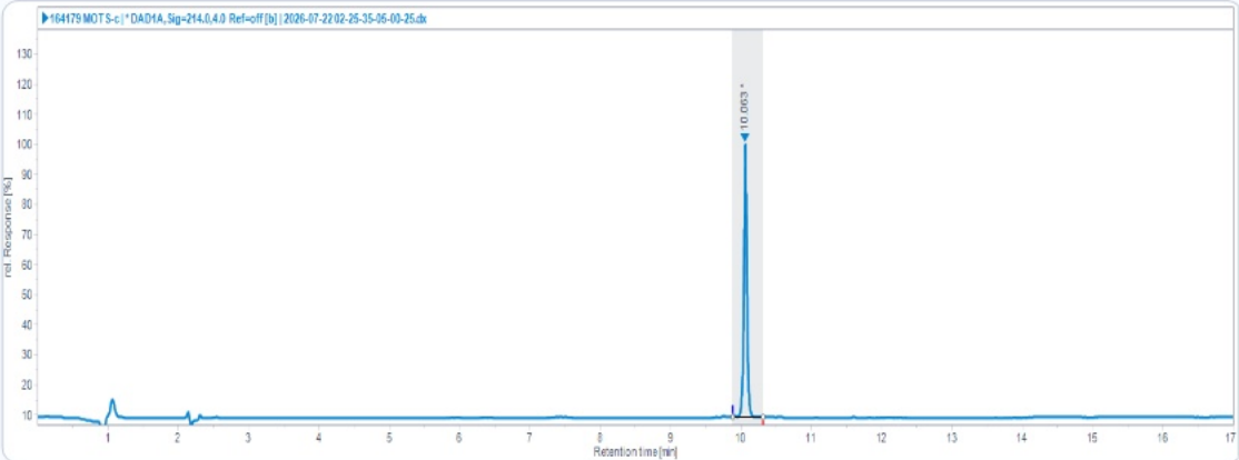
HPLC Chromatogram (Retention Time: 10.063 min)
