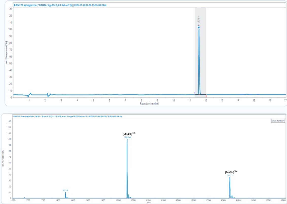
HPLC Chromatogram (Retention Time: 11.576 min)
