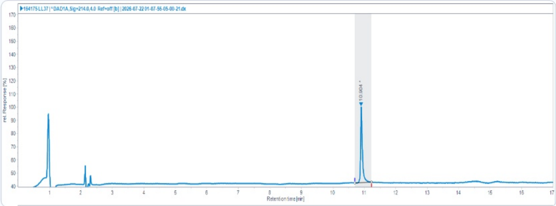
HPLC Chromatogram (Retention Time: 10.904 min)
