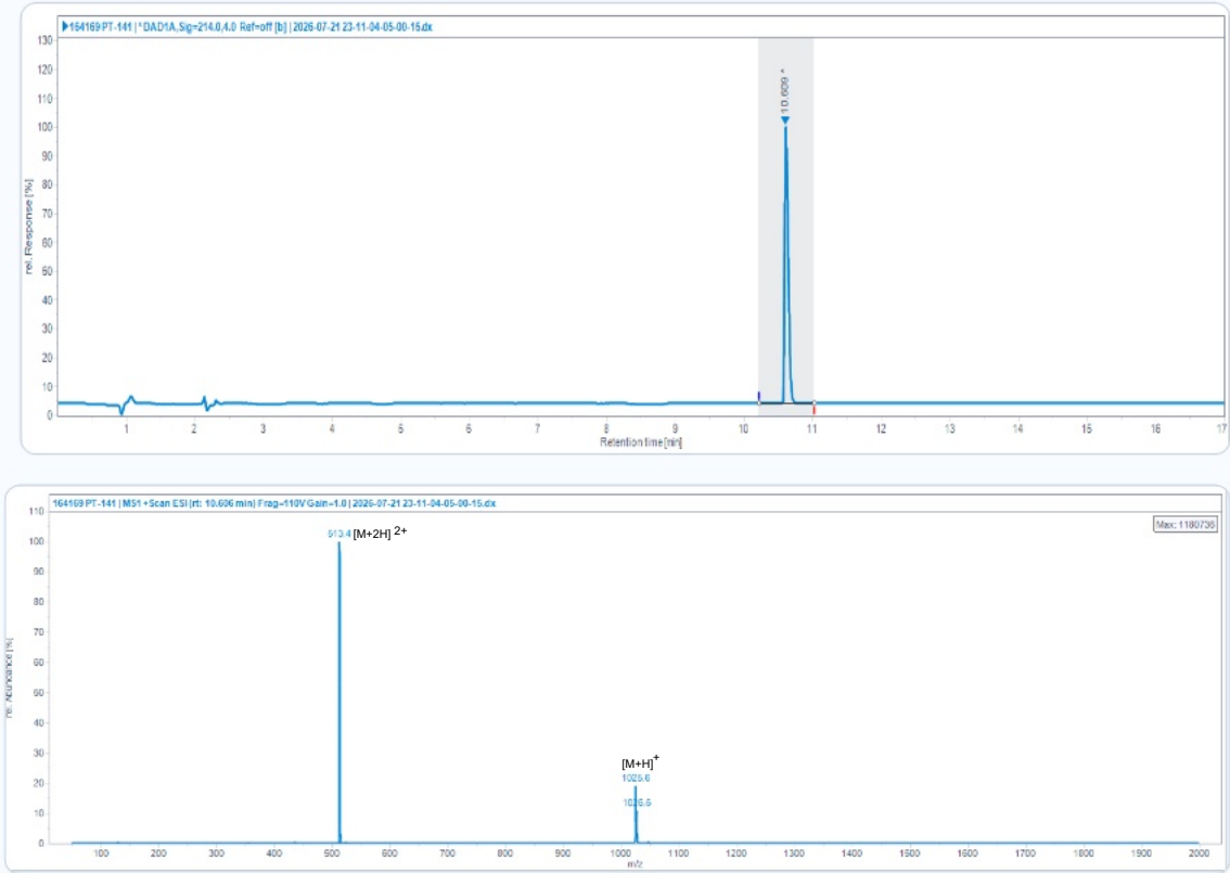
HPLC Chromatogram (Retention Time: 10.609 min)
