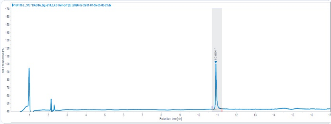
HPLC Chromatogram (Retention Time: 10.904 min)
