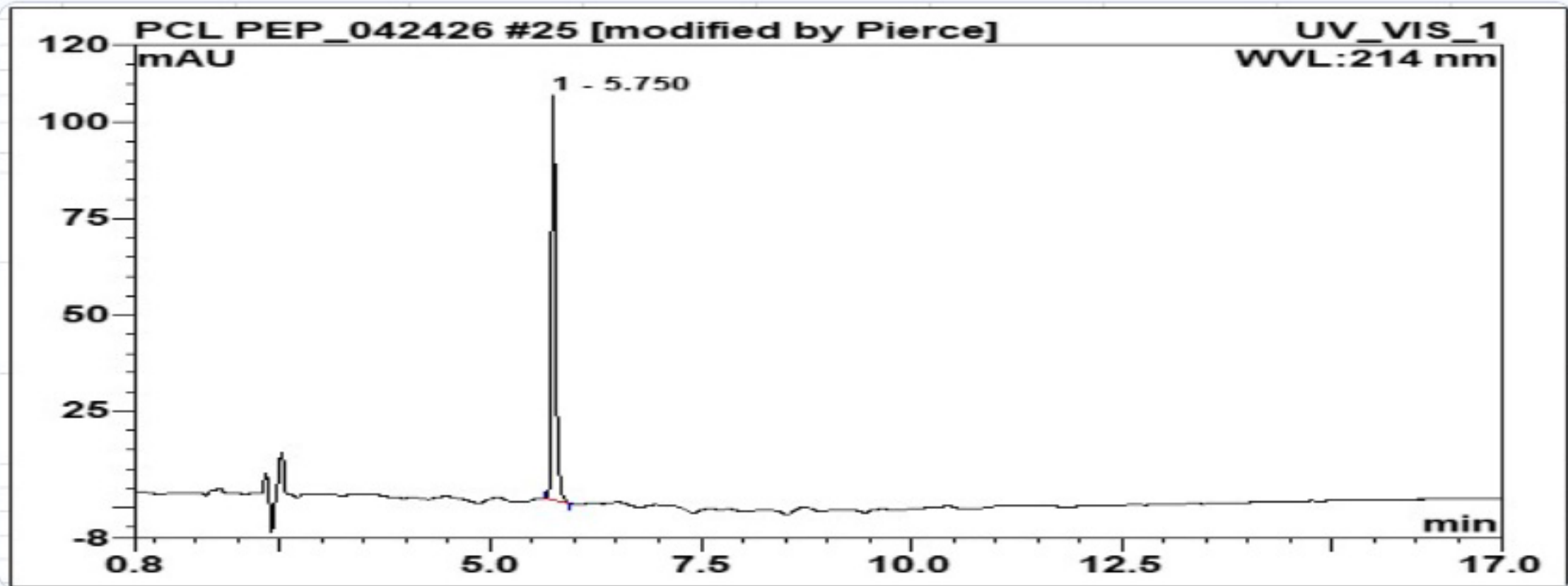
HPLC Chromatogram (Retention Time: 5.750 min)
