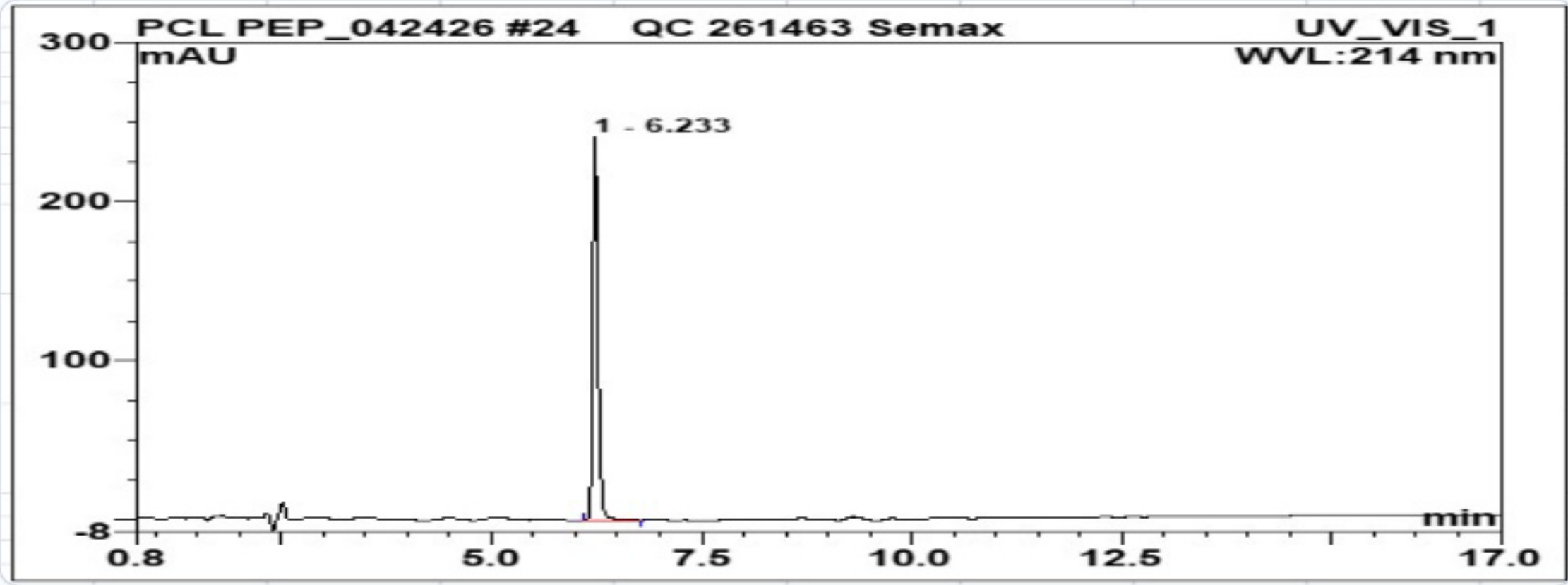
HPLC Chromatogram (Retention Time: 6.233 min)
