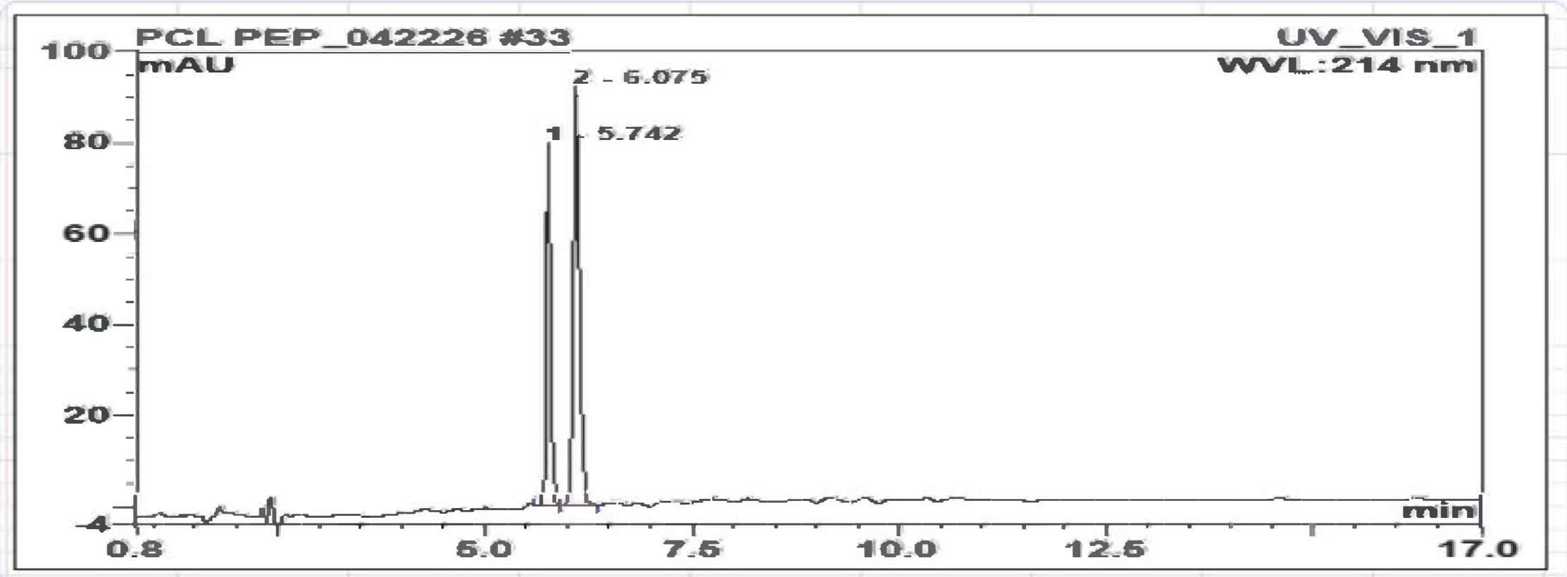
HPLC Chromatogram (Retention Time: 5.742, 6.075 min)
