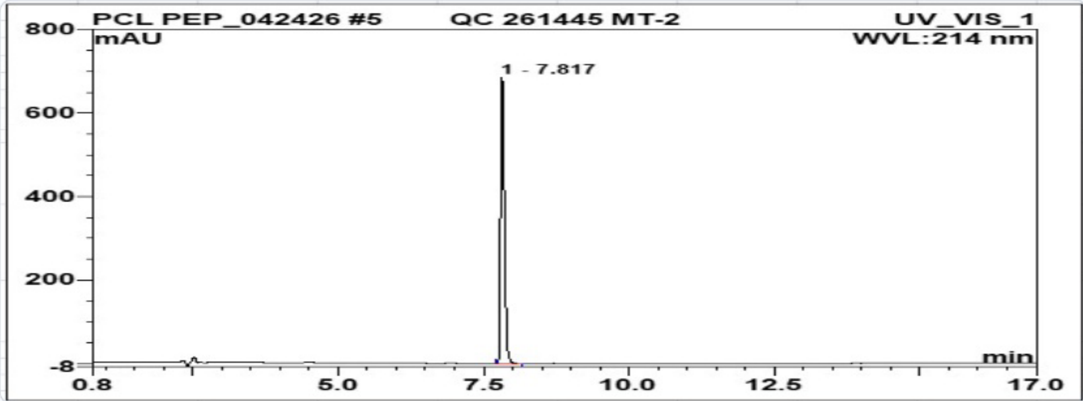
HPLC Chromatogram (Retention Time: 7.817 min)
