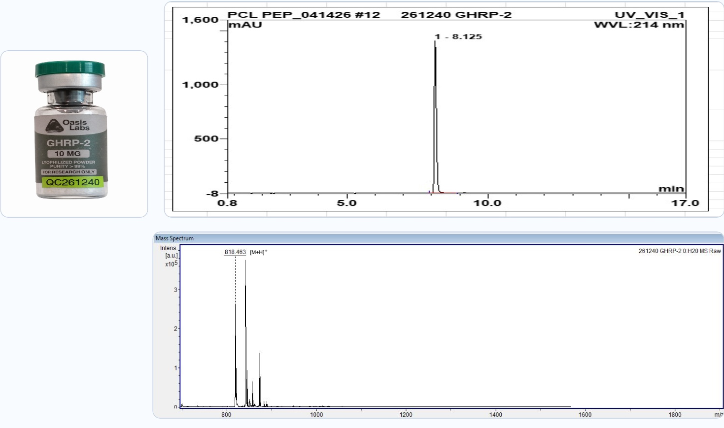
HPLC Chromatogram (Retention Time: 8.125 min)
